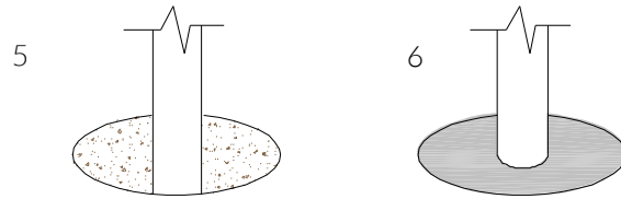
5 Compact base of hole with 50mm of aggregate. Lower ground Fix post attached to instrument straight and level before filling with concrete)
