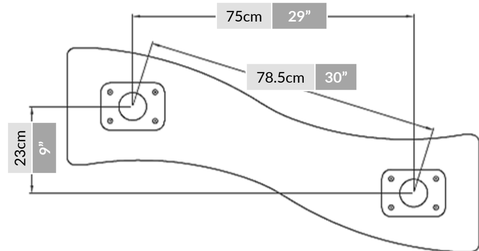
DUO SD Hole Centres
