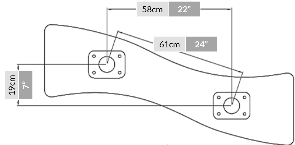
DUO HD Hole Centres
